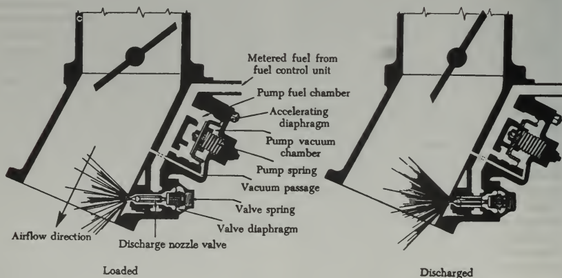
FIGURE 3-24. A single-diaphragm accelerating pump.
